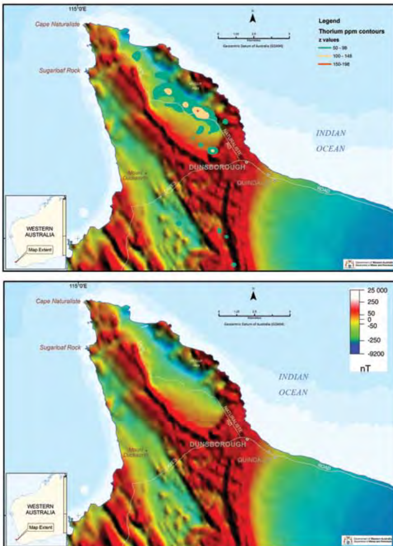
Figure 4 | Map showing the aeromagnetics in the vicinity of Dunsborough (Geological Survey of Western Australia, 2013) with the approximate location of the Th anomalies superimposed on the upper image. The lower image shows the aeromagnetics without the Th anomalies superimposed, and the colour scale of magnetic intensity in units of nanoTesla (nT). The magnitude of the Th anomalies in the upper image is represented as green indicating 50 to 100 ppm, light orange indicating 100 to 150 ppm, and red indicating 150 to 200 ppm. Ground measurements indicated Th concentrations in the order of 280 ppm in the light orange regions
