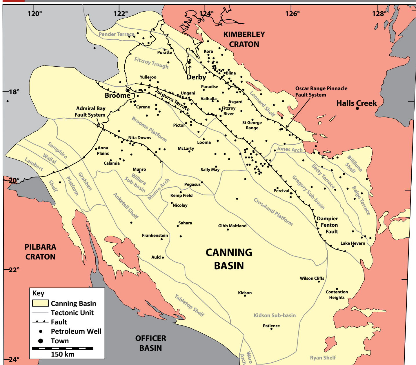
Figure 1 | Onshore Canning Basin, showing recently drilled wells
