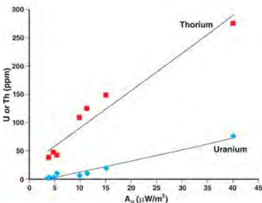
Figure 3 | Plot of heat generation ( A_0 in units of \mu\text{W/m}^3 ) versus U concentration (blue diamonds), and Th (red squares) for the various locations investigated in the Leeuwin Complex (see Figure 1 for locations). The figure shows that heat generation varies between 3.8 and 40.1 \mu\text{W/m}^3 . Linear regression lines are shown for both elements (U and Th) versus the heat generation ( A_0 )
