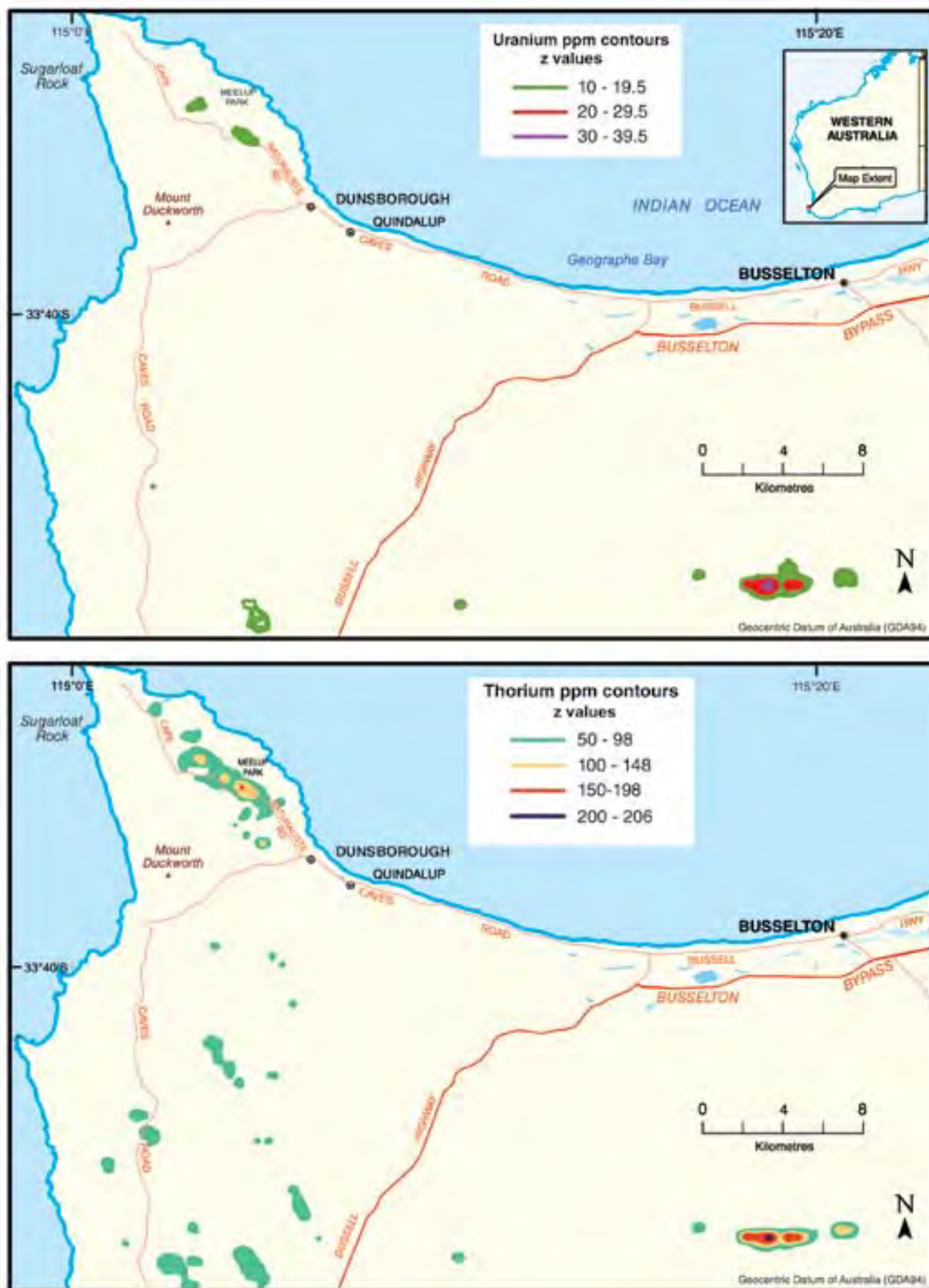
Figure 2 | Maps showing (a) U concentrations and (b) Th concentrations in the northern Vasse region, based on airborne radiometric data
