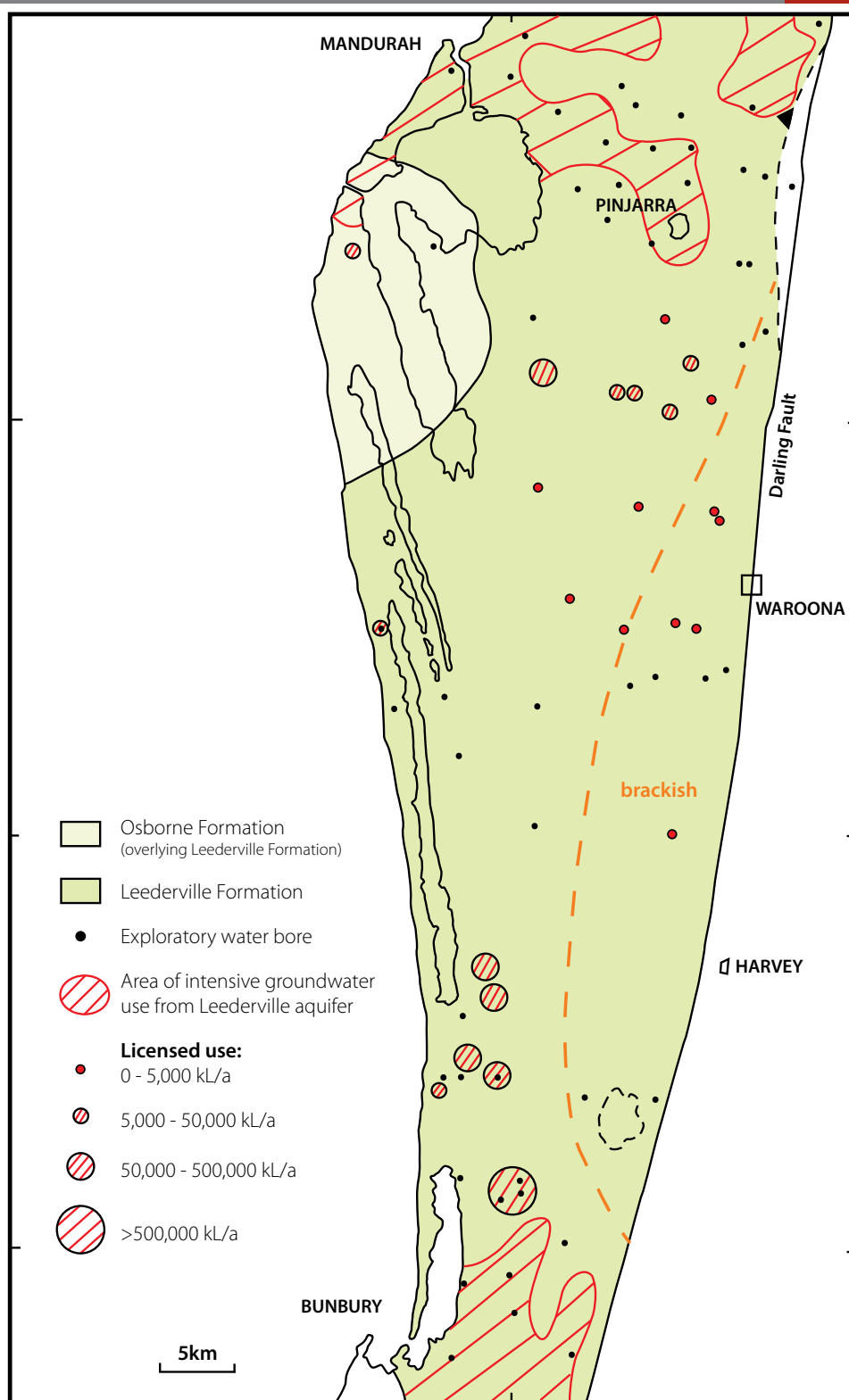
Figure 2 | Leederville aquifer
